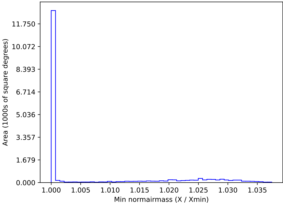
weather_cloudso30v3.4_10yrs WFD z band: Min normairmass
