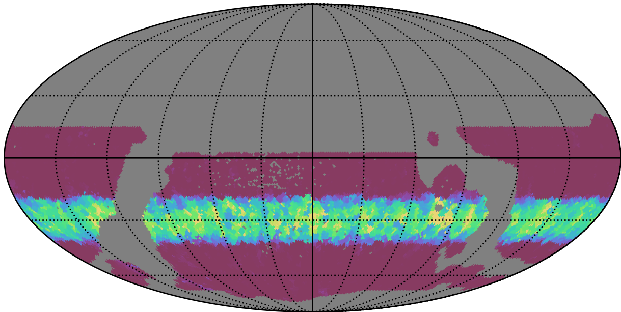
weather_cloudso30v3.4_10yrs WFD u band: Min normairmass
