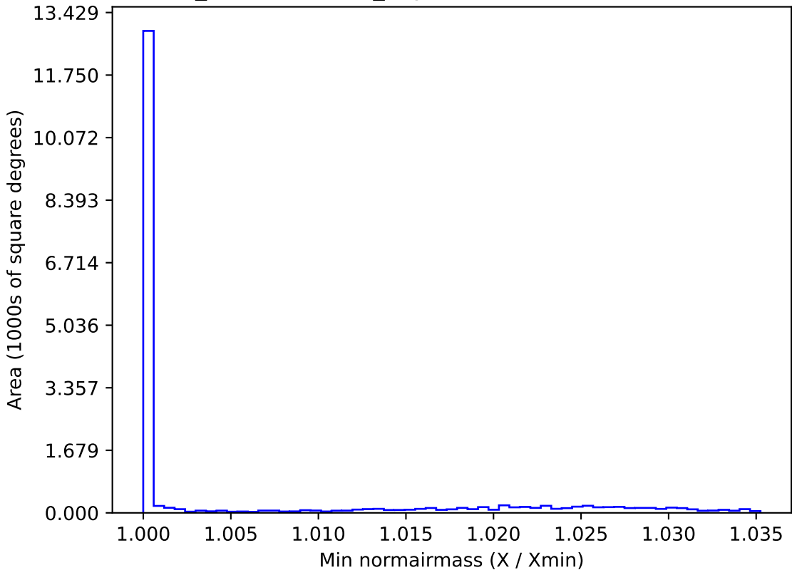
weather_cloudso30v3.4_10yrs WFD r band: Min normairmass
