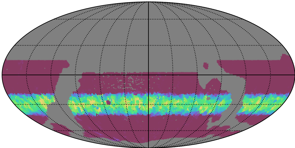
weather_cloudso30v3.4_10yrs WFD g band: Min normairmass
