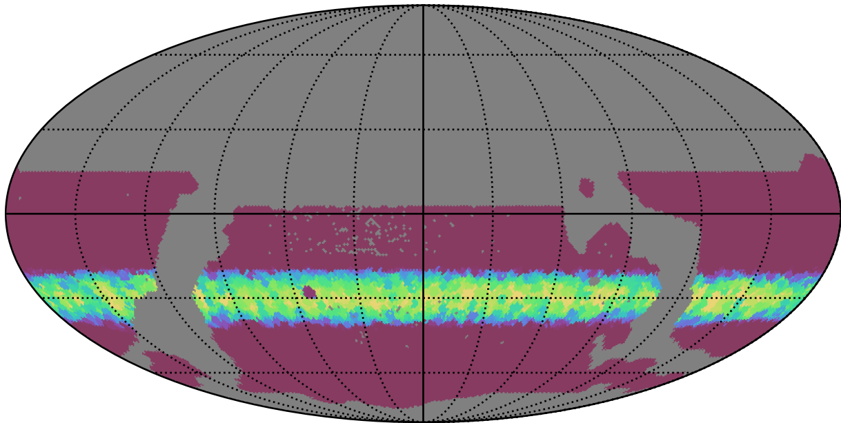
weather_cloudso30v3.4_10yrs WFD all bands: Min normairmass
