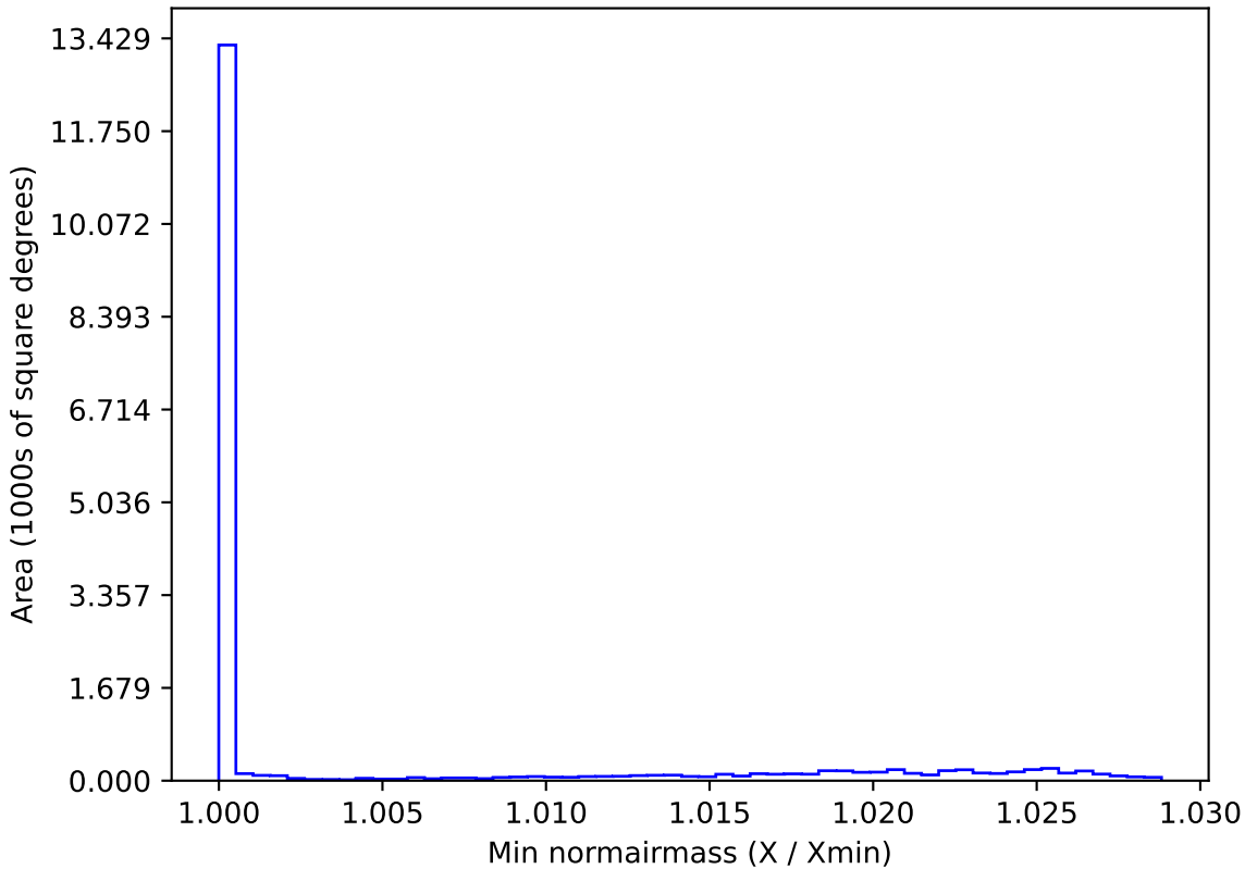
weather_cloudso30v3.4_10yrs WFD all bands: Min normairmass
