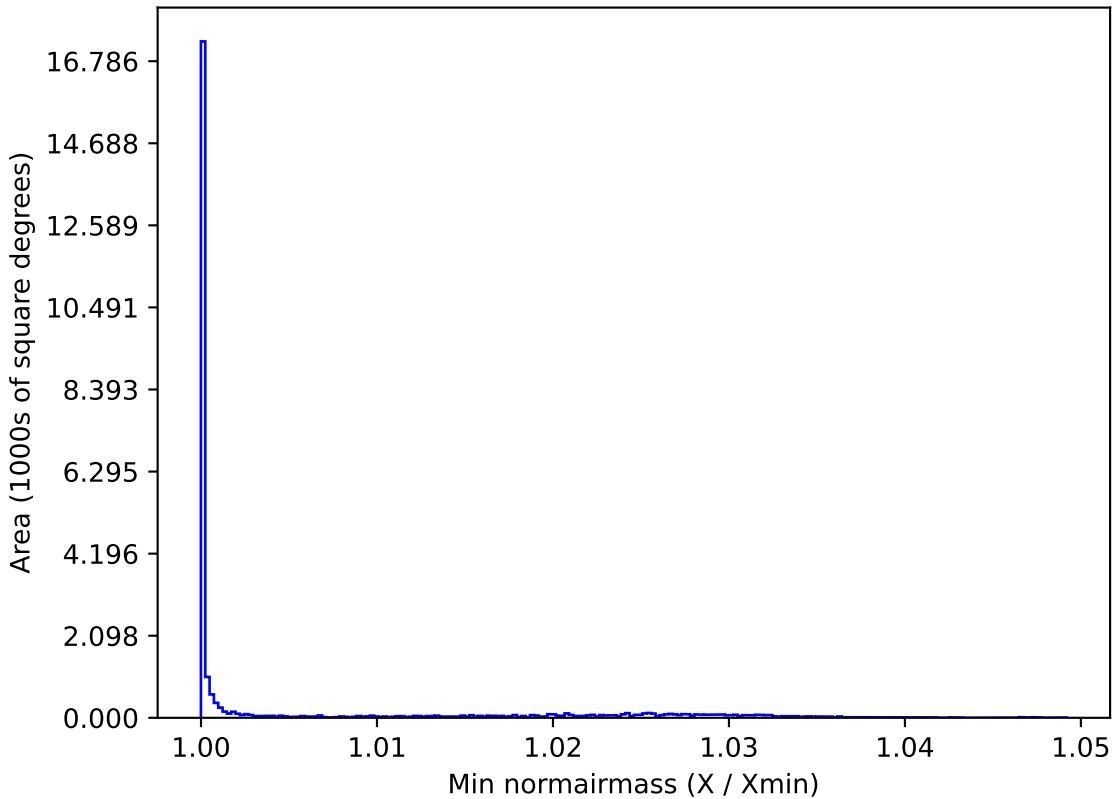
weather_cloudso30v3.4_10yrs All sky z band: Min normairmass
