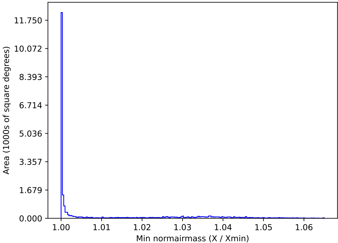
weather_cloudso30v3.4_10yrs All sky u band: Min normairmass
