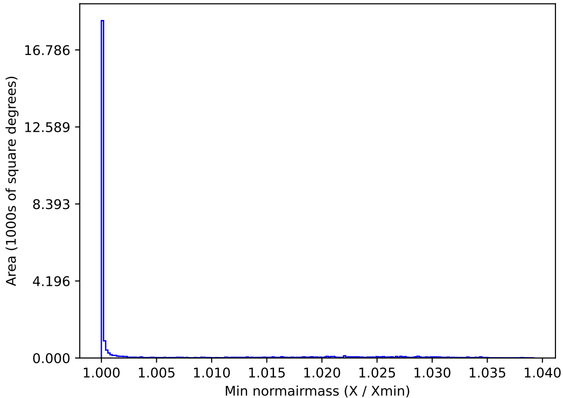
weather_cloudso30v3.4_10yrs All sky r band: Min normairmass
