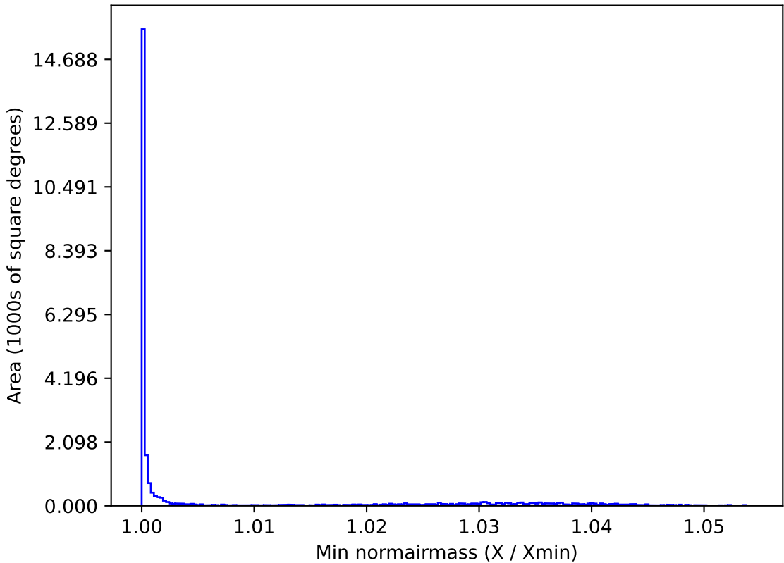
weather_cloudso30v3.4_10yrs All sky g band: Min normairmass
