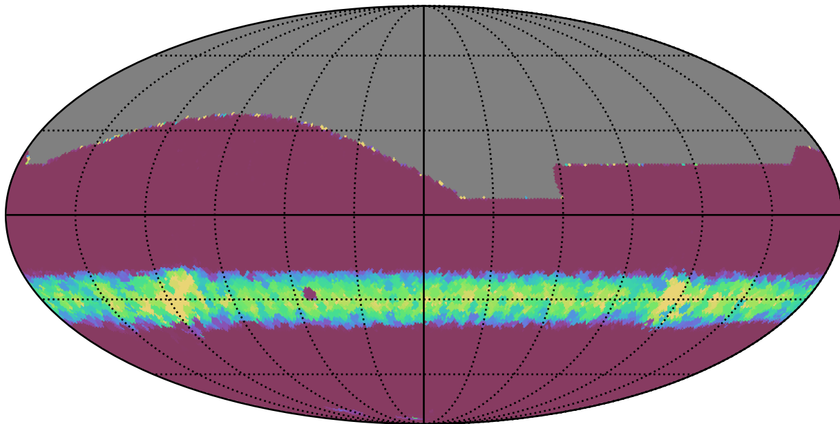
weather_cloudso30v3.4_10yrs All sky all bands: Min normairmass
