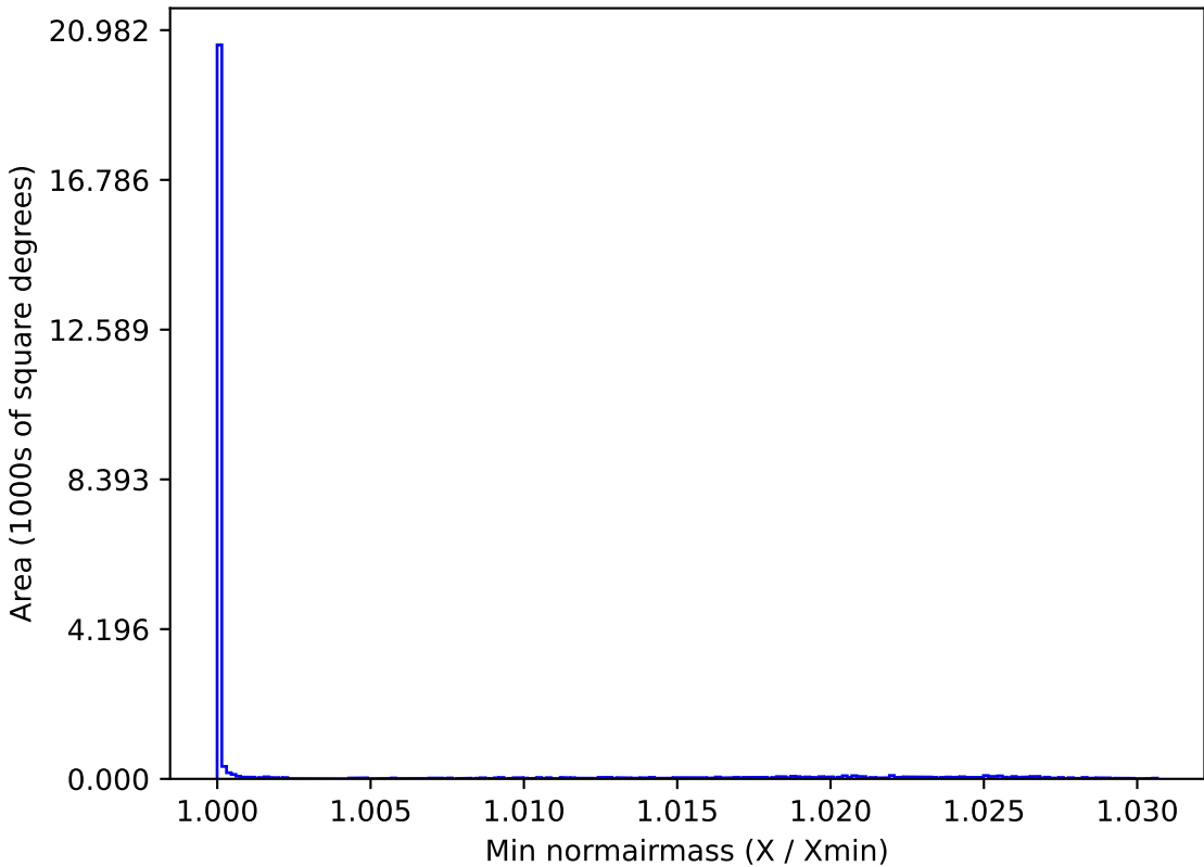
weather_cloudso30v3.4_10yrs All sky all bands: Min normairmass
