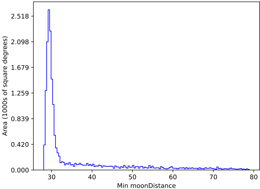
weather_cloudso30v3.4_10yrs WFD y band: Min moonDistance
