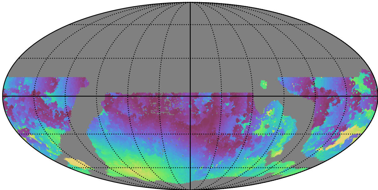
weather_cloudso30v3.4_10yrs WFD u band: Min moonDistance
