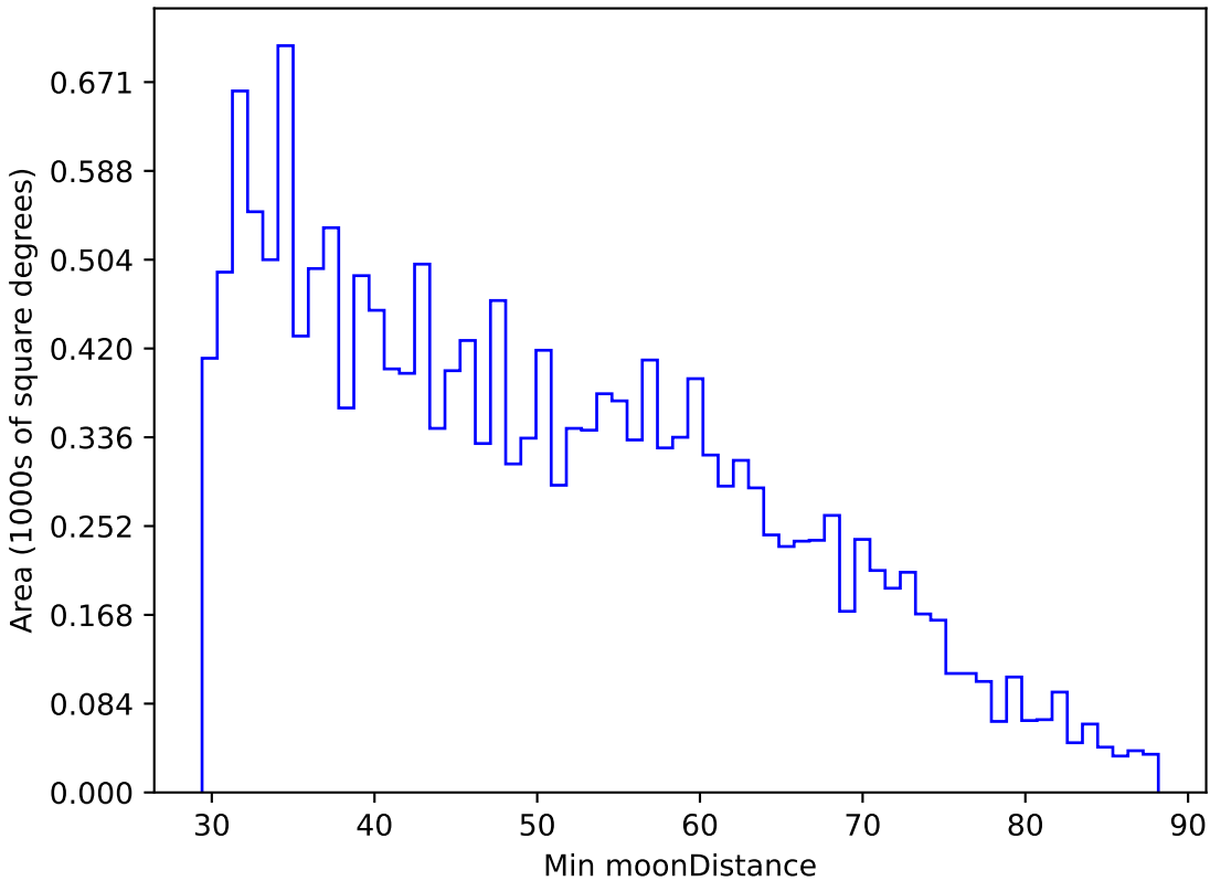
weather_cloudso30v3.4_10yrs WFD u band: Min moonDistance
