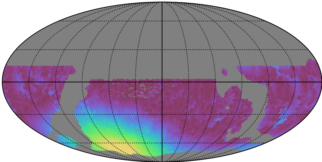
weather_cloudso30v3.4_10yrs WFD r band: Min moonDistance
