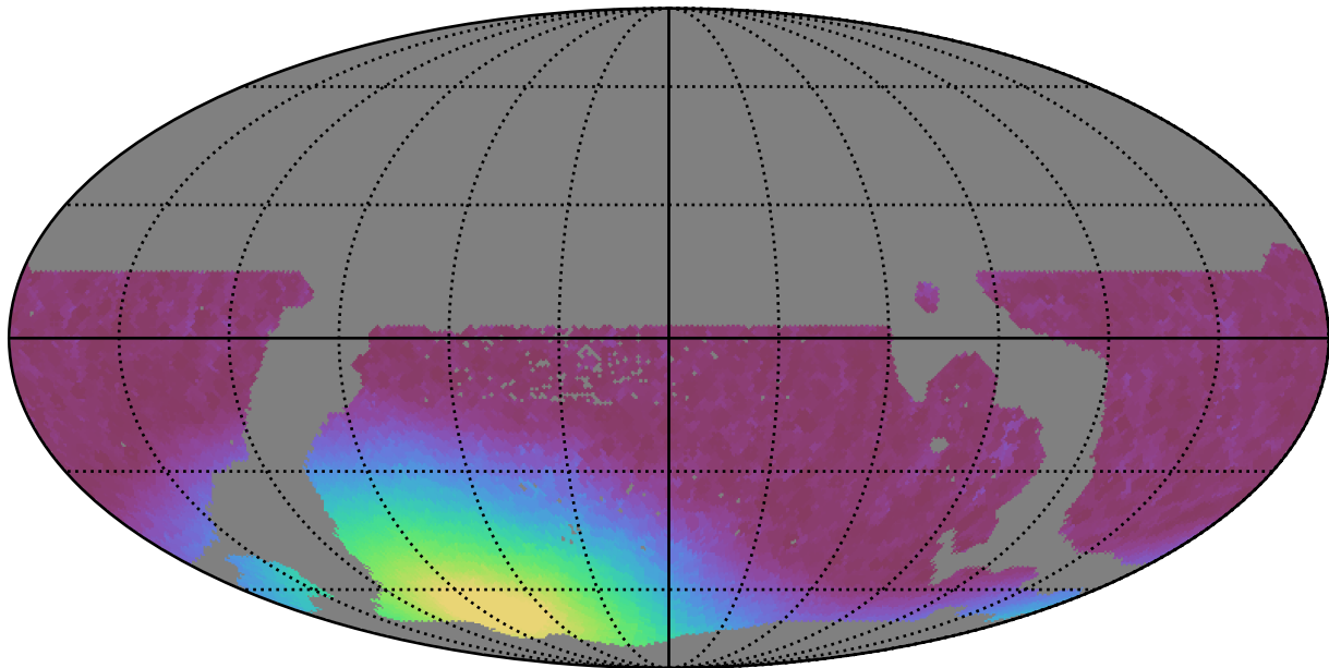
weather_cloudso30v3.4_10yrs WFD i band: Min moonDistance
