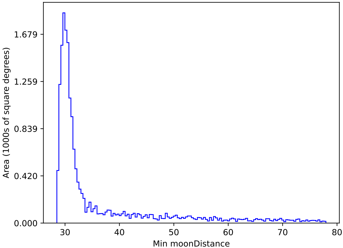
weather_cloudso30v3.4_10yrs WFD i band: Min moonDistance
