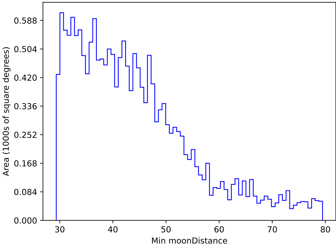
weather_cloudso30v3.4_10yrs WFD g band: Min moonDistance
