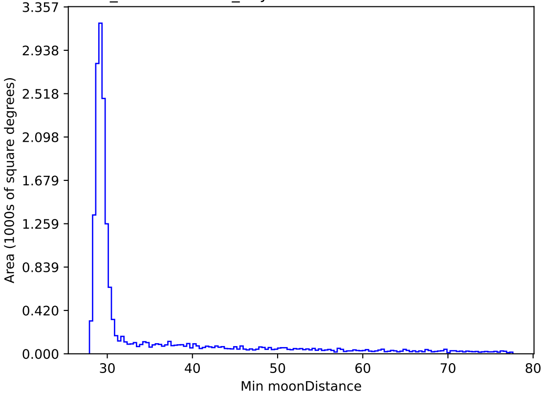
weather_cloudso30v3.4_10yrs WFD all bands: Min moonDistance
