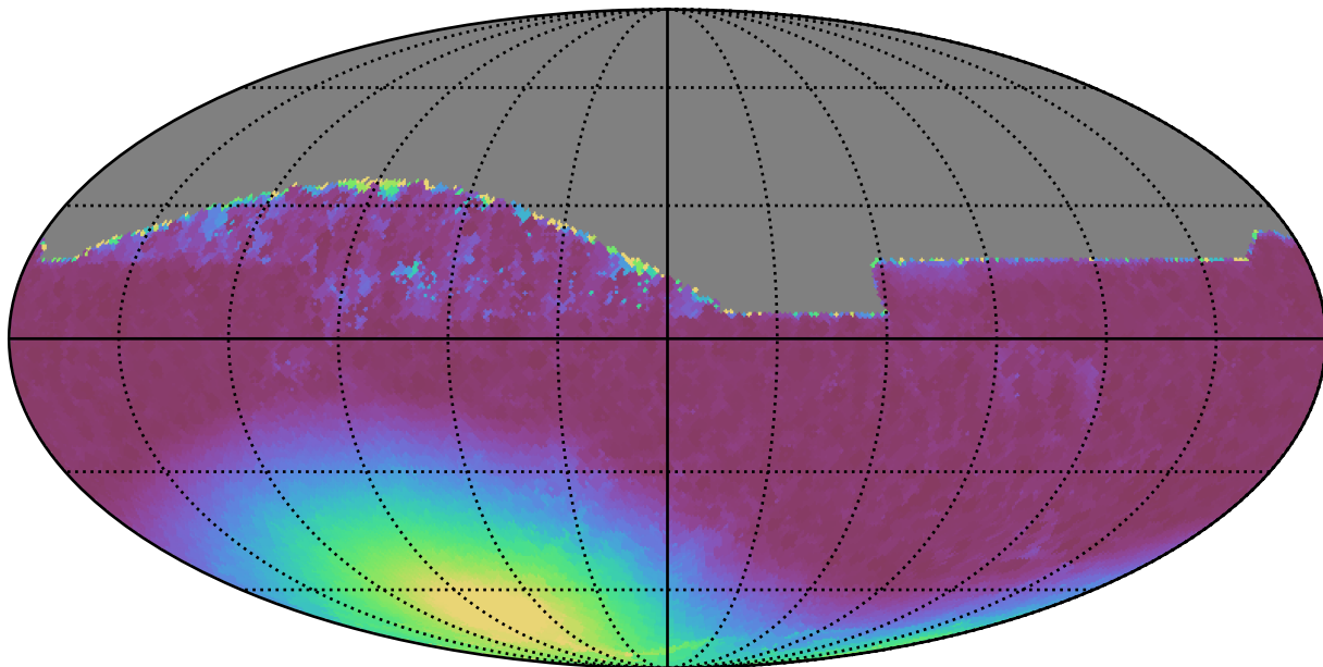
weather_cloudso30v3.4_10yrs All sky z band: Min moonDistance
