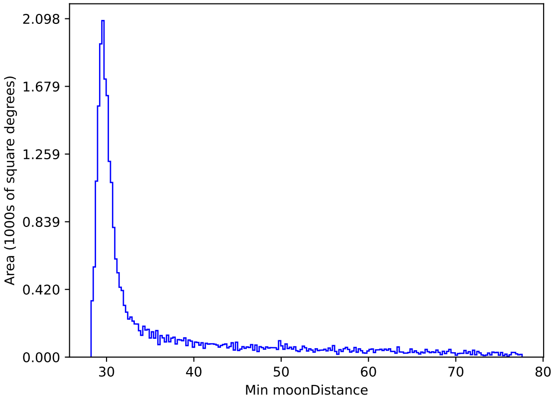
weather_cloudso30v3.4_10yrs All sky z band: Min moonDistance
