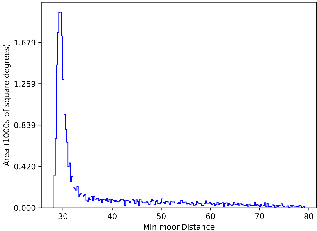
weather_cloudso30v3.4_10yrs All sky y band: Min moonDistance
