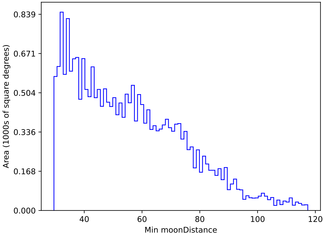
weather_cloudso30v3.4_10yrs All sky u band: Min moonDistance
