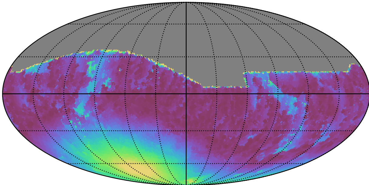
weather_cloudso30v3.4_10yrs All sky r band: Min moonDistance
