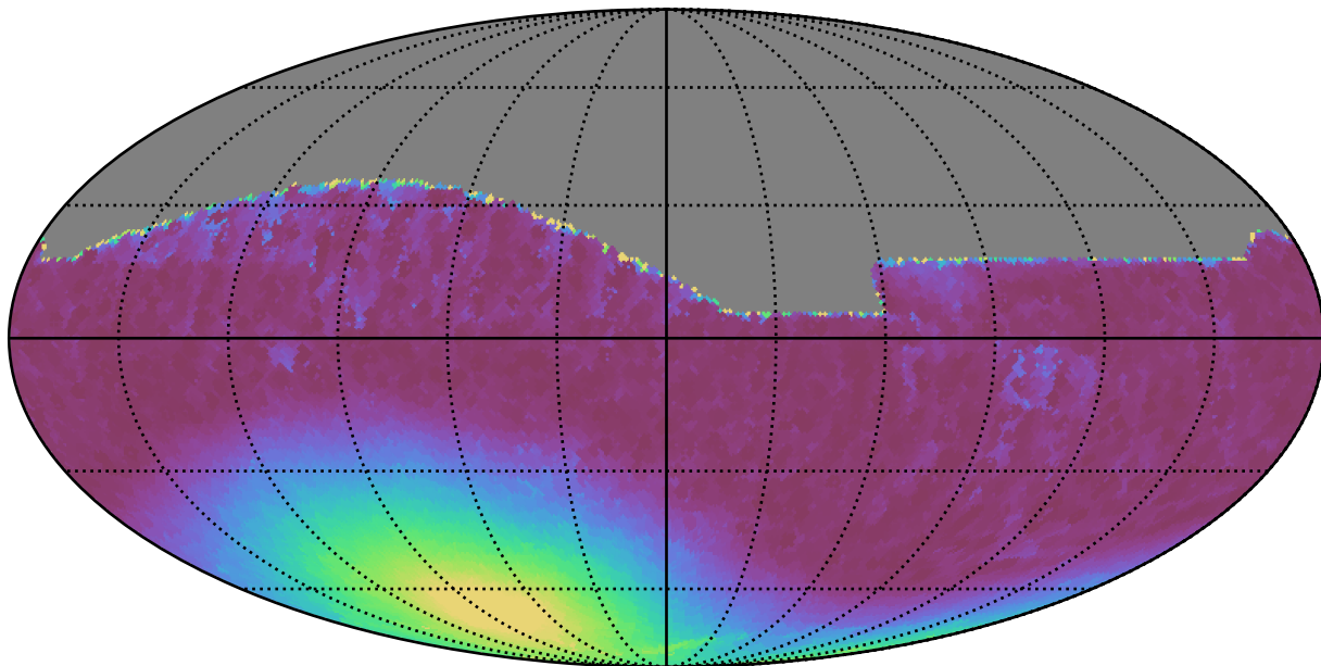
weather_cloudso30v3.4_10yrs All sky i band: Min moonDistance
