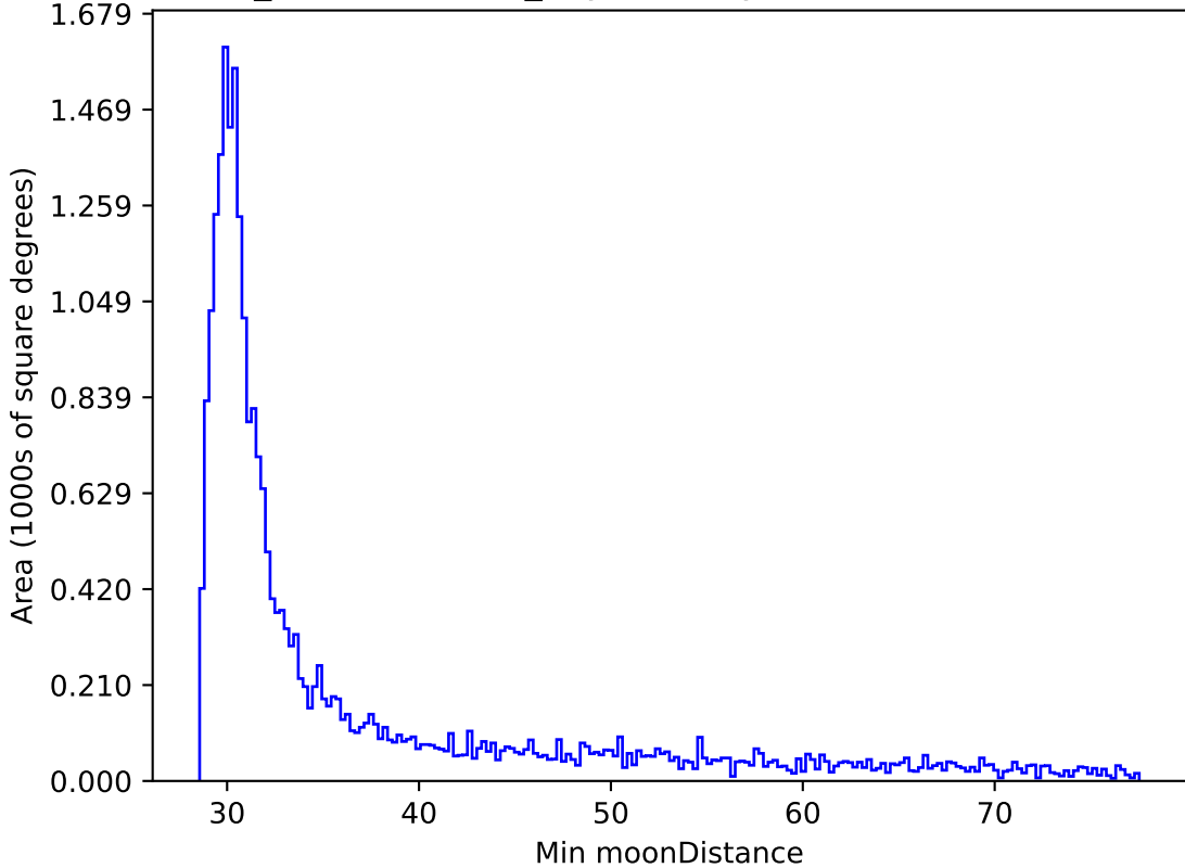
weather_cloudso30v3.4_10yrs All sky i band: Min moonDistance
