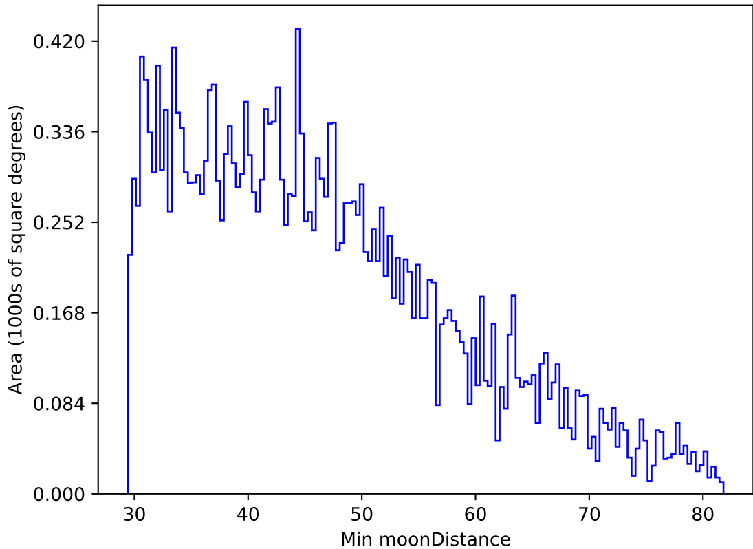
weather_cloudso30v3.4_10yrs All sky g band: Min moonDistance
