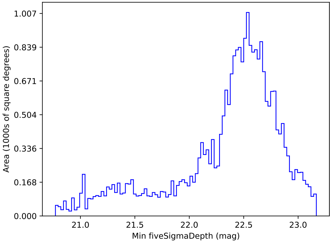
weather_cloudso30v3.4_10yrs Yr 1 z band: Min fiveSigmaDepth
