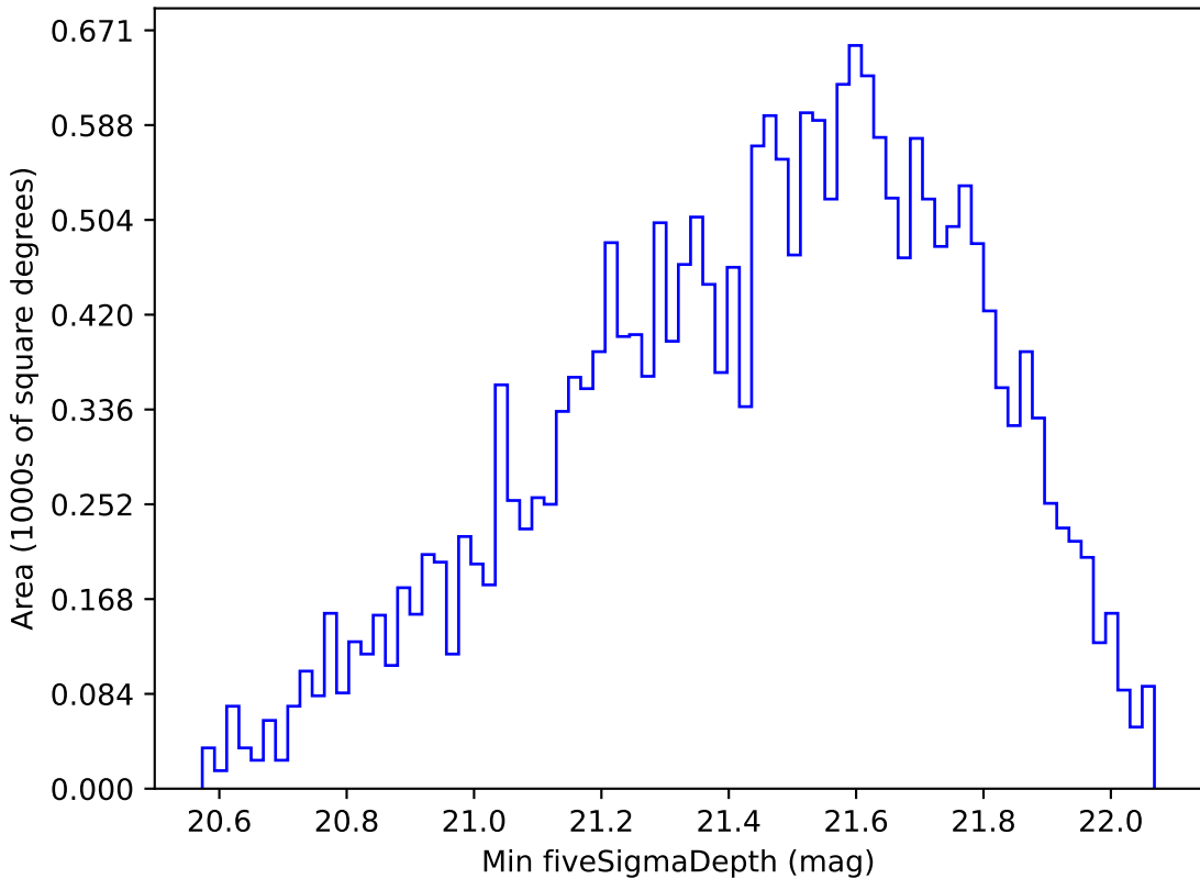
weather_cloudso30v3.4_10yrs Yr 1 y band: Min fiveSigmaDepth
