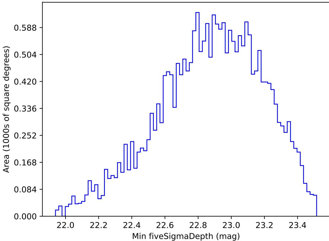
weather_cloudso30v3.4_10yrs Yr 1 u band: Min fiveSigmaDepth
