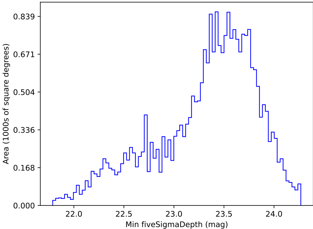
weather_cloudso30v3.4_10yrs Yr 1 r band: Min fiveSigmaDepth
