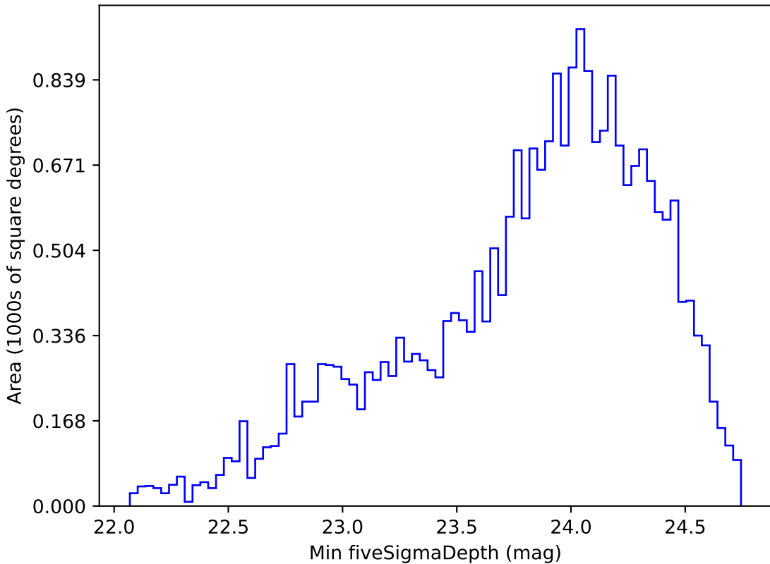
weather_cloudso30v3.4_10yrs Yr 1 g band: Min fiveSigmaDepth
