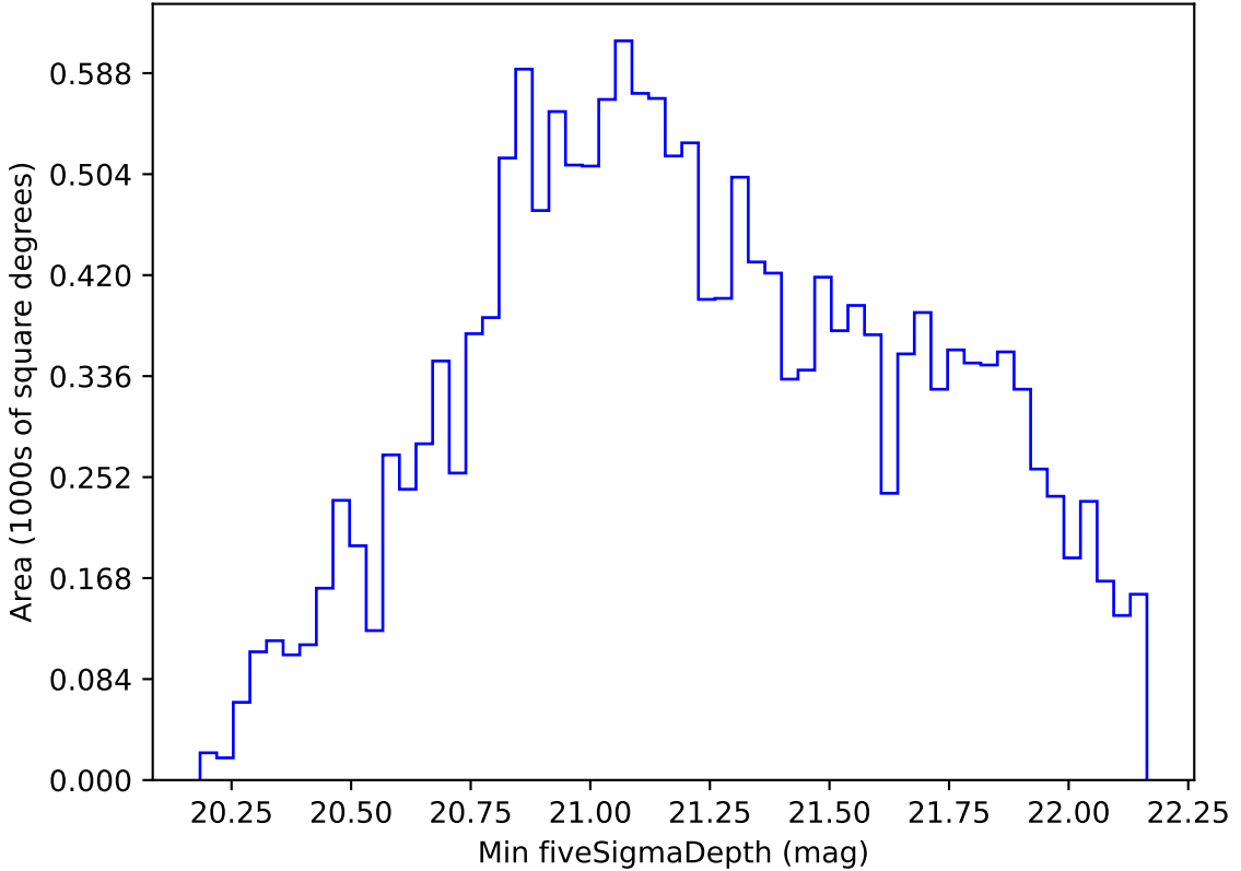
weather_cloudso30v3.4_10yrs WFD z band: Min fiveSigmaDepth
