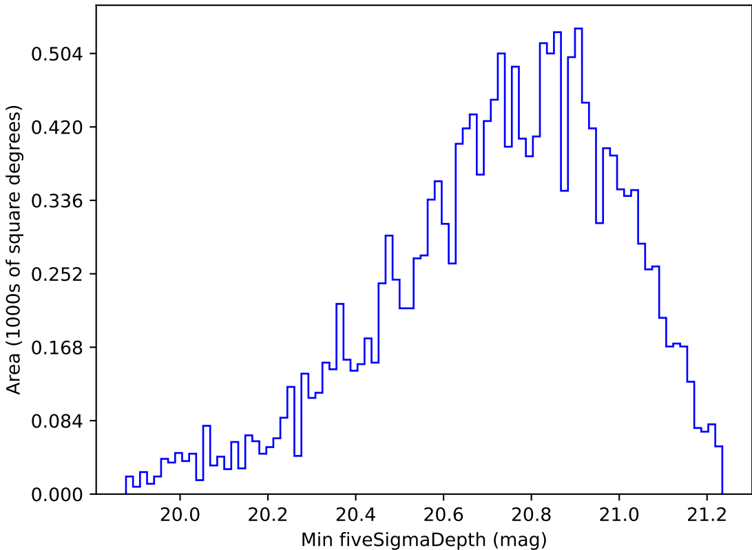
weather_cloudso30v3.4_10yrs WFD y band: Min fiveSigmaDepth
