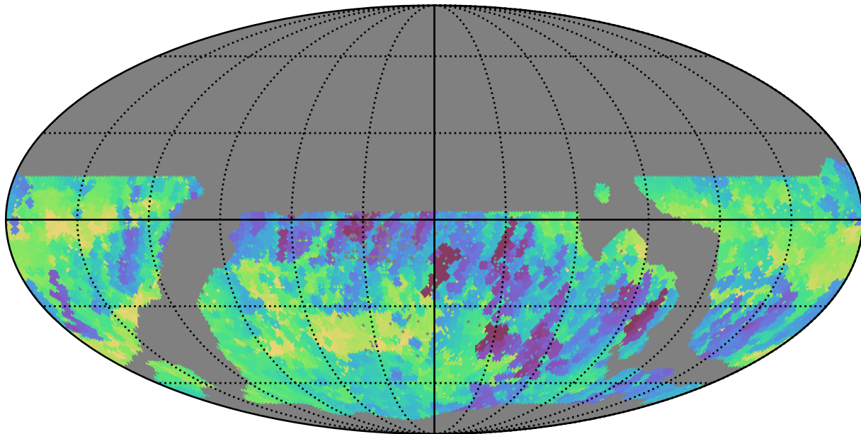
weather_cloudso30v3.4_10yrs WFD r band: Min fiveSigmaDepth
