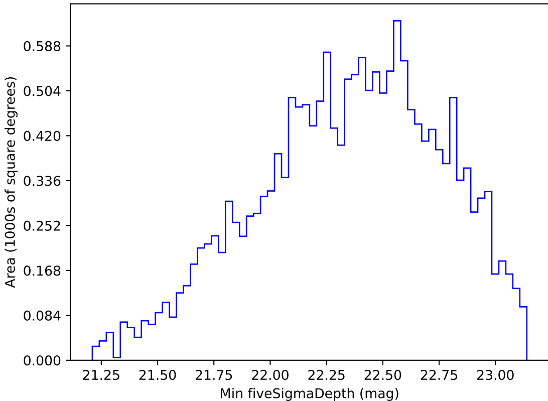
weather_cloudso30v3.4_10yrs WFD r band: Min fiveSigmaDepth
