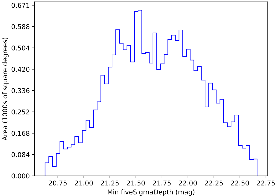
weather_cloudso30v3.4_10yrs WFD i band: Min fiveSigmaDepth
