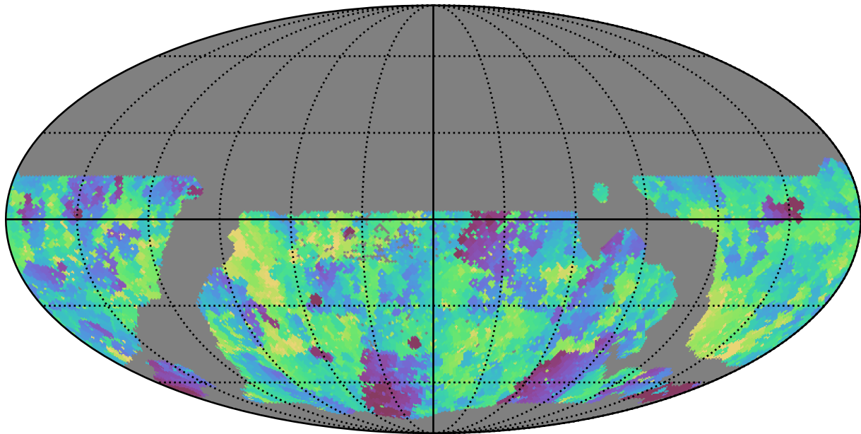
weather_cloudso30v3.4_10yrs WFD g band: Min fiveSigmaDepth
