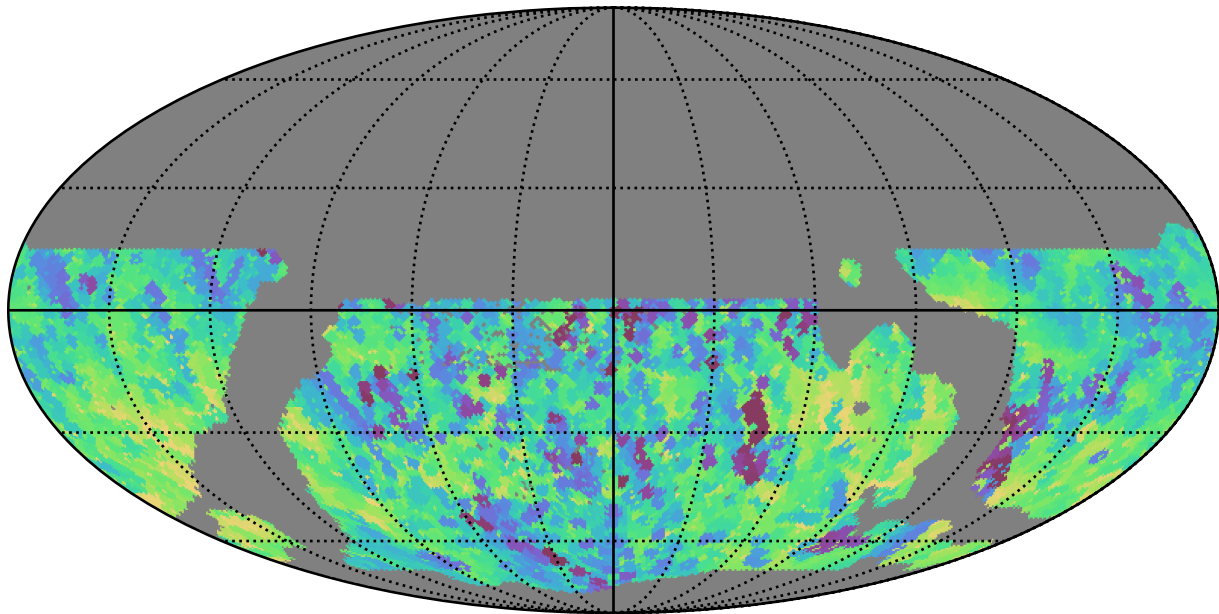
weather_cloudso30v3.4_10yrs WFD all bands: Min fiveSigmaDepth
