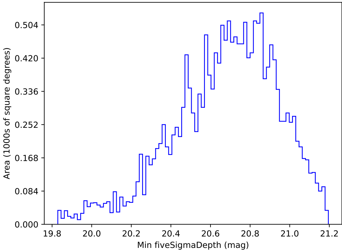
weather_cloudso30v3.4_10yrs WFD all bands: Min fiveSigmaDepth
