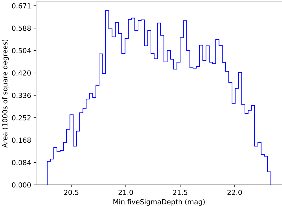
weather_cloudso30v3.4_10yrs All sky z band: Min fiveSigmaDepth
