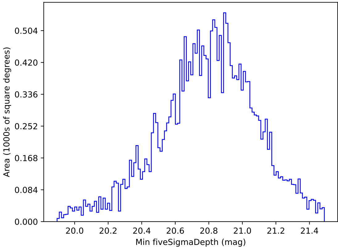
weather_cloudso30v3.4_10yrs All sky y band: Min fiveSigmaDepth
