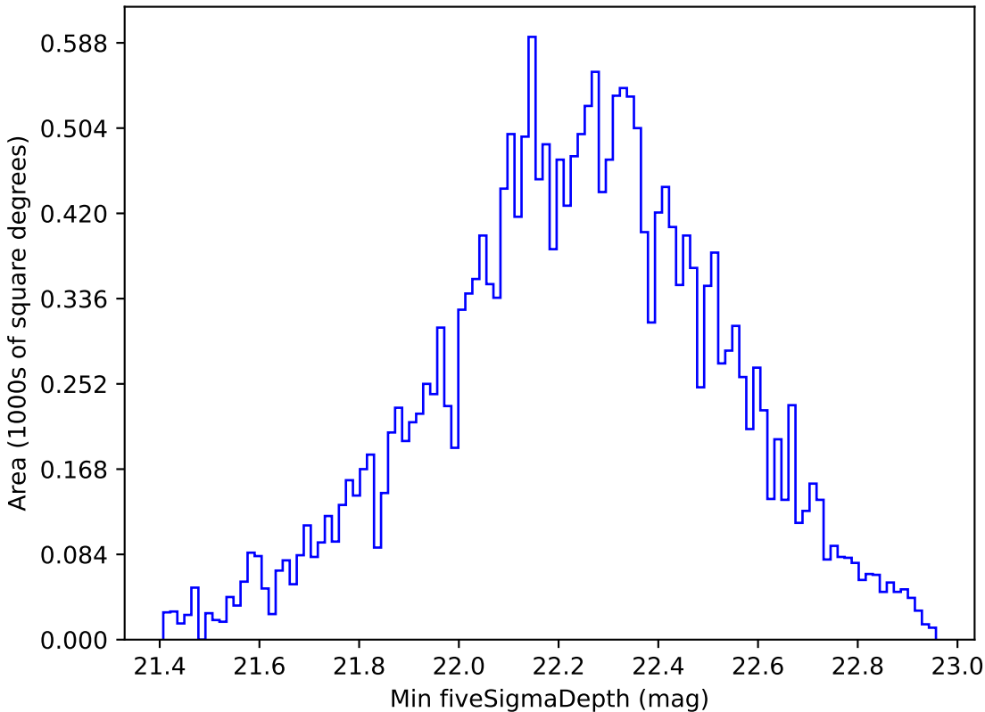
weather_cloudso30v3.4_10yrs All sky u band: Min fiveSigmaDepth
