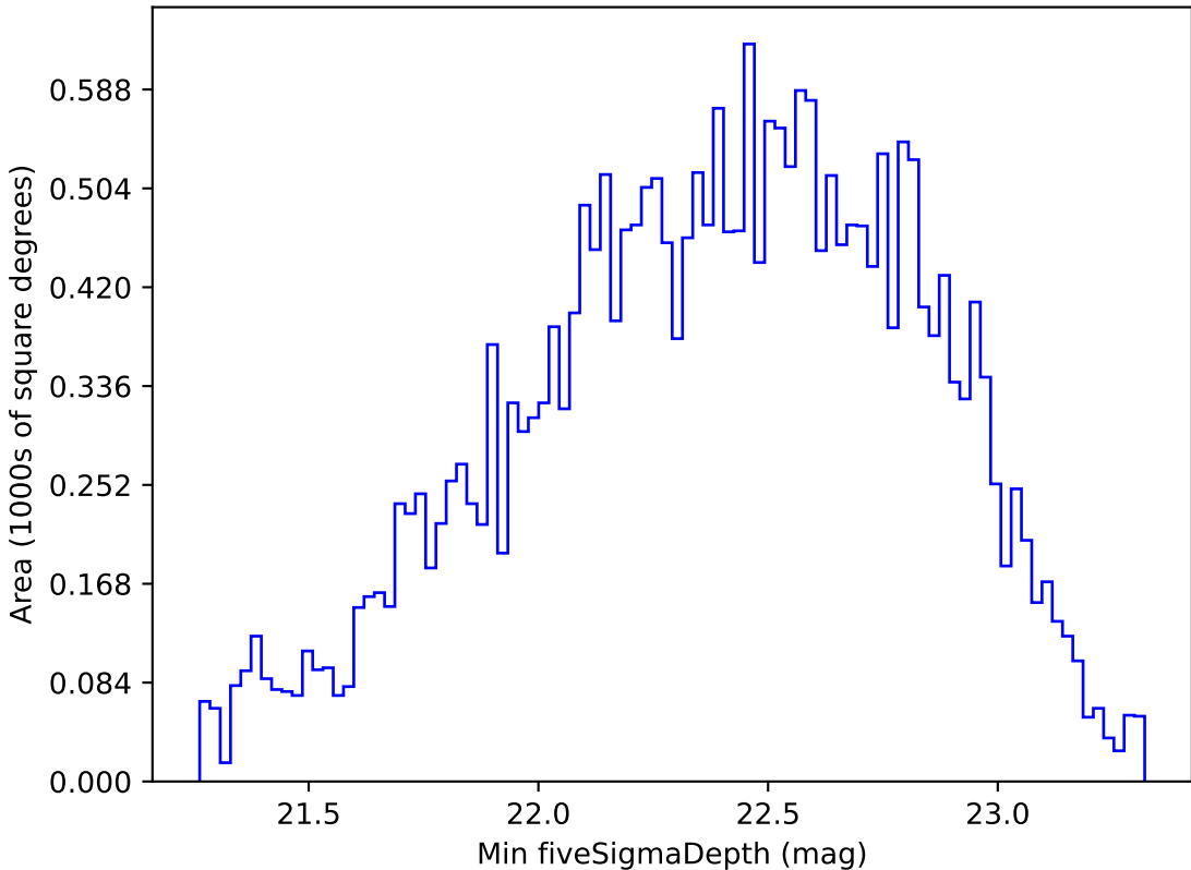
weather_cloudso30v3.4_10yrs All sky r band: Min fiveSigmaDepth
