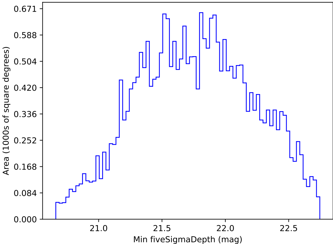
weather_cloudso30v3.4_10yrs All sky i band: Min fiveSigmaDepth
