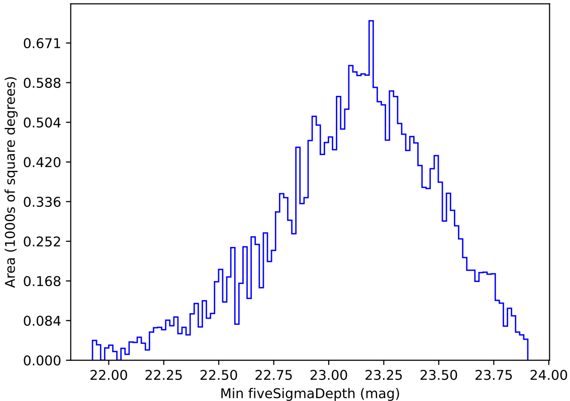
weather_cloudso30v3.4_10yrs All sky g band: Min fiveSigmaDepth
