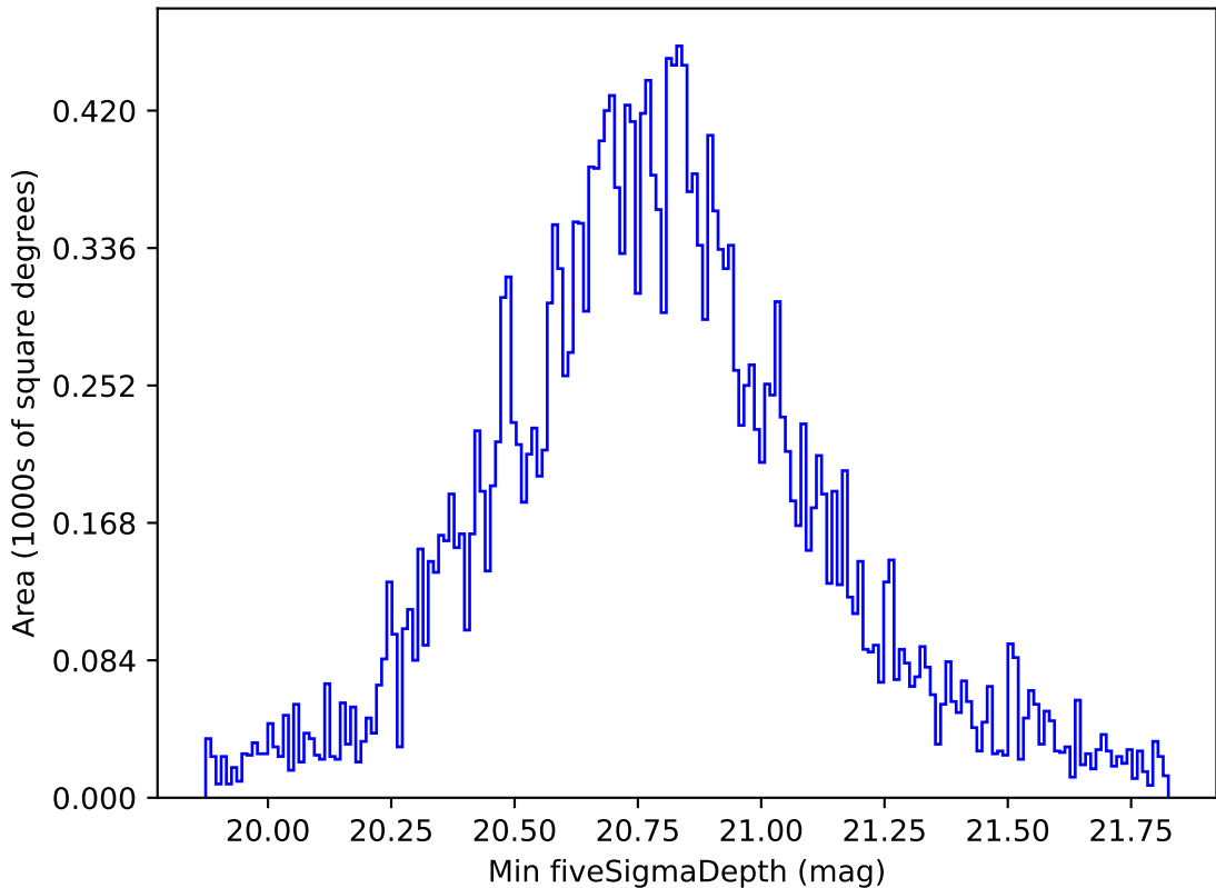
weather_cloudso30v3.4_10yrs All sky all bands: Min fiveSigmaDepth
