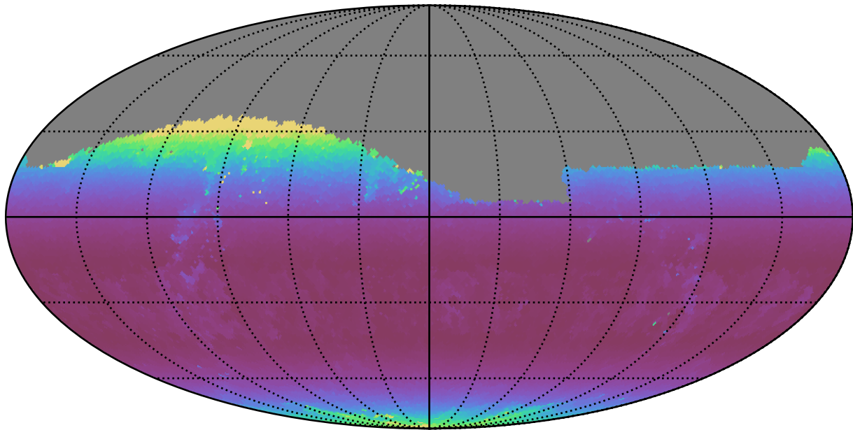
weather_cloudso30v3.4_10yrs Yr 1 z band: Min airmass
