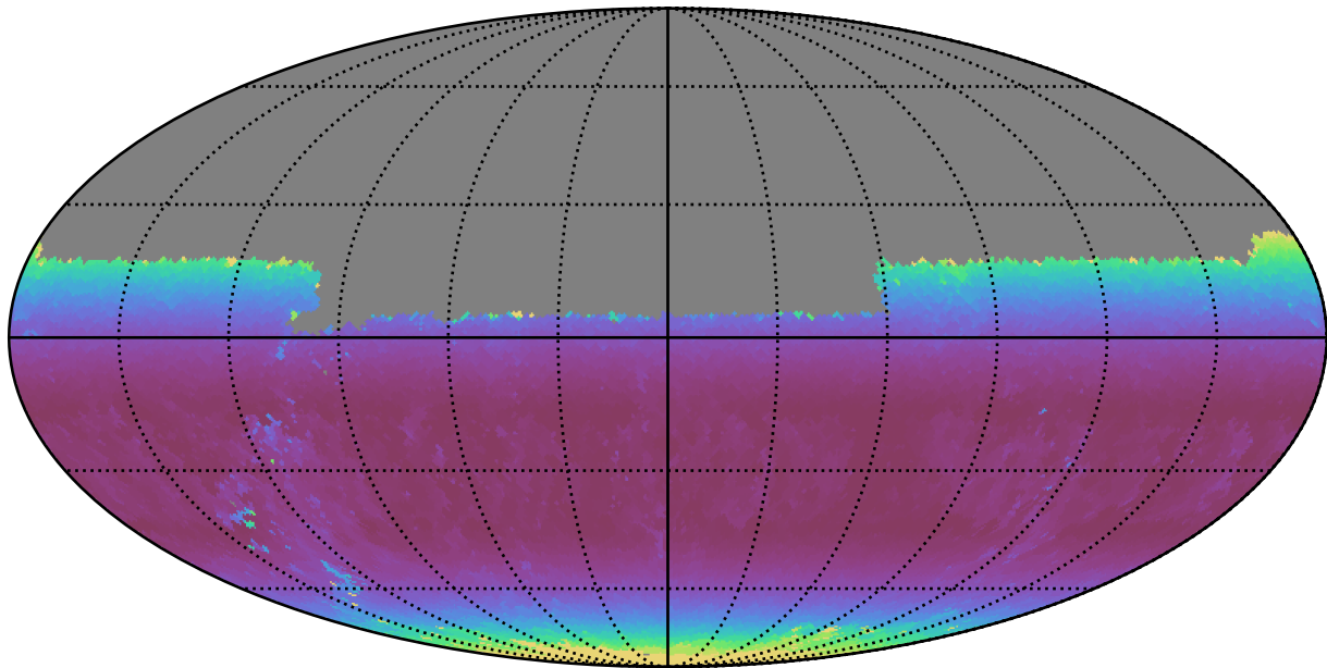
weather_cloudso30v3.4_10yrs Yr 1 y band: Min airmass
